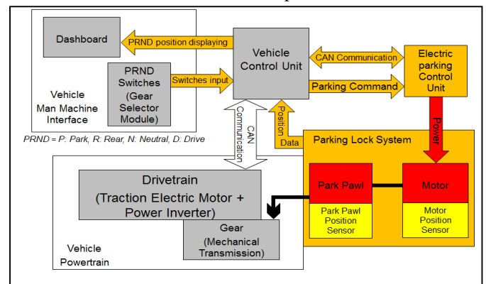
Fig. 1. Electric parking system function blocks
